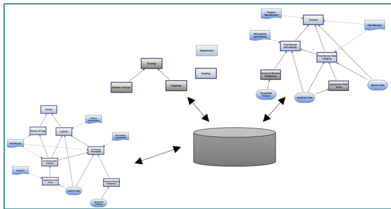
Multiple Decision Models Share A Common Repository Maximizing Coverage and Reuse
